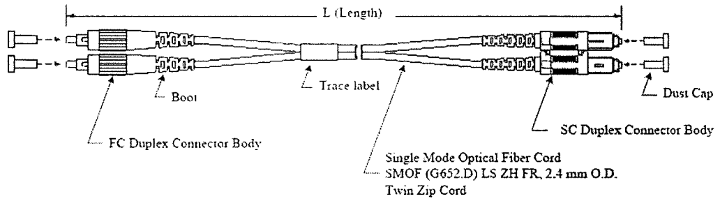
Figure 12 FC to SC Single Mode Fiber Patch Cord Duplex
